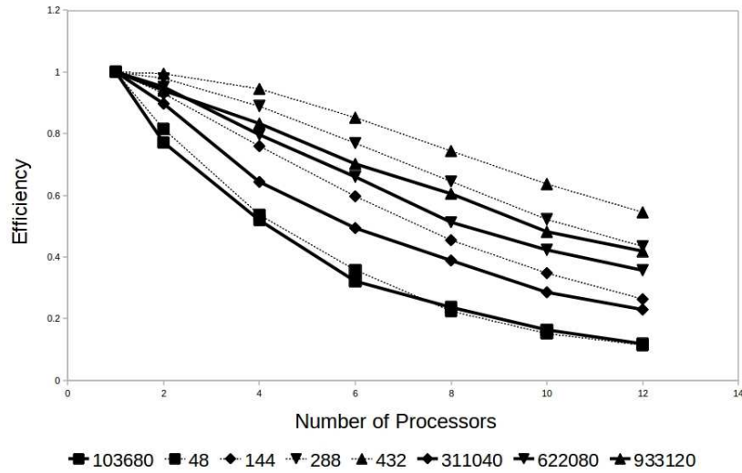
Figure 10: Efficiencies comparison of the data growing towards landscape and portrait format. The efficiencies for the yeast data are plotted in the top half of the figure and the efficiencies for the diabetes data are plotted in the bottom half of the figure.
