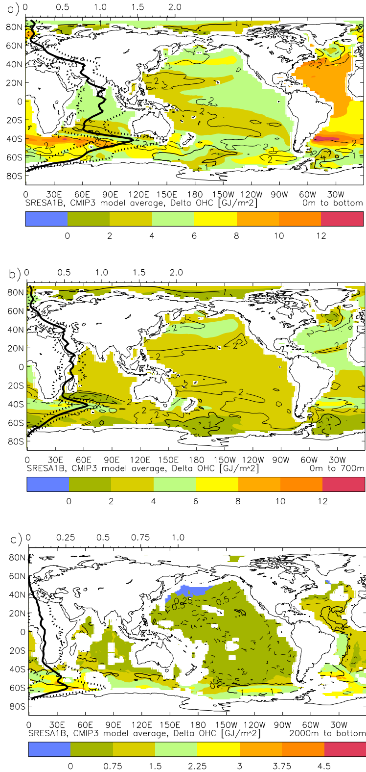
Figure 4. Vertically integrated ocean heat uptake (colour shading; in GJ m -2 ) in the ensemble average of the SRES A1B scenario of 17 CMIP3 models for (a) the total water column, (b) the upper 700 m and (c) below 2000 m. Thick black line: zonal total in 10 15 J m -1 (scale in the upper left corner), with \pm 1 standard deviation (dotted). Note the different scales in Figure 4c. Black contours show the ratio R of ensemble mean and ensemble standard deviation (solid: R > 1 , thick solid: R = 1 , dashed: R < 1 ). For Figures 4a and 4b, R > 1 in most areas indicating agreement across models. An exception are the deep-water formation regions in the Southern Ocean and the North Atlantic. In Figure 4c the models mainly show OHU in the Southern Ocean.
