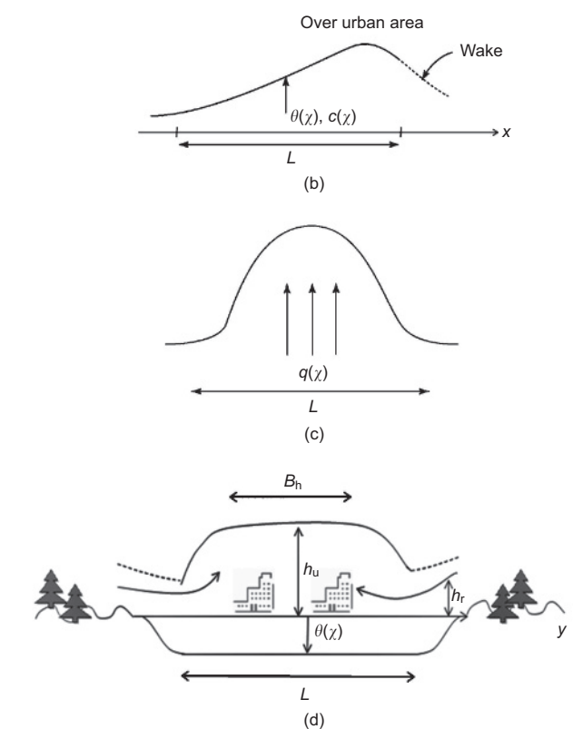
Figure 3. Some schematic features of the atmospheric environment of large cities. (a) Airflow patterns when the diameter L becomes comparable with L_R (the Rossby radius – deformation over which the flow is influenced upwind and in the wake downwind \sim 30 km at night). (b) Typical asymmetrical variation of mean temperature \theta(x) of non-reactive pollutant c(x) when wind is from left to right (variation is quite different for reactive pollutants). (c) Typical vertical flux of mean temperature or pollutant. (d) Looking downwind (i.e. in x direction) showing how at night the wind passes over the urban area and the surface urban temperature \theta(x) is raised over the entire width L , but as the cool rural air moves inwards the width B_h is less than L . The boundary layer depth h_u is significantly greater than the rural boundary layer depth h_r (see Figures 1 and 2)
