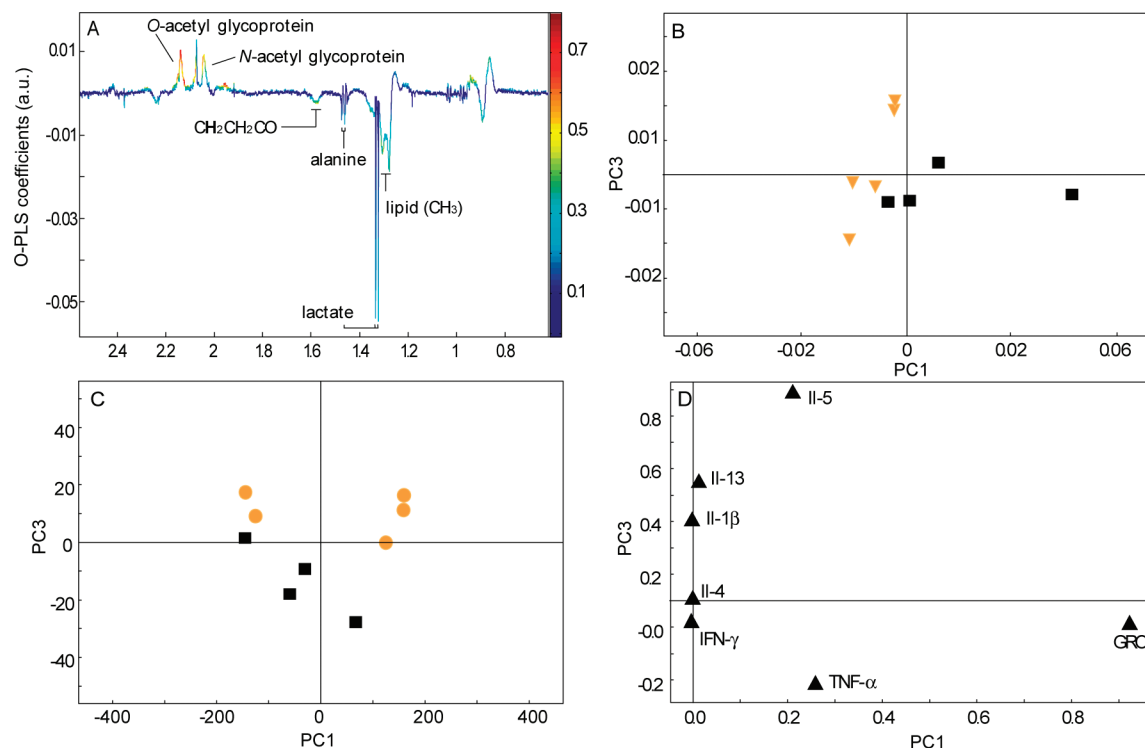
Figure 2. Differentiation of plasma samples obtained from a pairwise comparison of plasma ^1\text{H} NMR data of F. hepatica -infected vs. noninfected control rats at day 22 postinfection. (A) O-PLS-DA coefficient plot; (B) PCA of ^1\text{H} NMR plasma data; (C) PCA scores plot; and (D) PCA coefficients plot based on the relative levels of selected cytokines assessed on day 22 postinfection in F. hepatica -infected rats (orange) and noninfected control rats (black).
