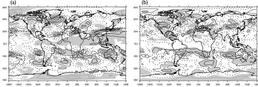
Figure 3: Trends in blended tropopause height (a) DJF and (b) JJA for ERA-Interim (1989-2007). Solid contours show positive trends, the zero line is dashed, and negative contours are dotted. The contour interval is 100 \text{ m decade}^{-1} . Shading highlights where the trends are significant at or above the 5% level.
