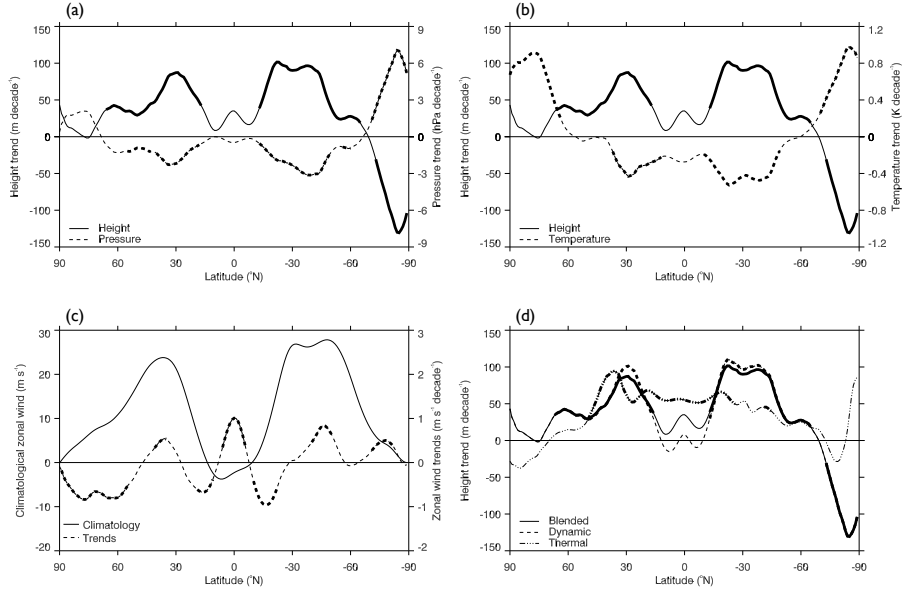
Figure 1: (a) Annual-mean zonal-mean blended tropopause height and pressure trends ( \text{m decade}^{-1} and \text{hPa decade}^{-1} ) from ERA-Interim (1989-2007). (b) Tropopause height and temperature trends ( \text{m decade}^{-1} and \text{K decade}^{-1} ). (c) Tropopause level zonal-mean zonal wind climatology and trends ( \text{m s}^{-1} and \text{m s}^{-1} \text{ decade}^{-1} ). (d) Annual-mean zonal-mean blended, dynamic and thermal tropopause height ( \text{m decade}^{-1} ). Bold lines indicate where trends are significant at or above the 5% level.
