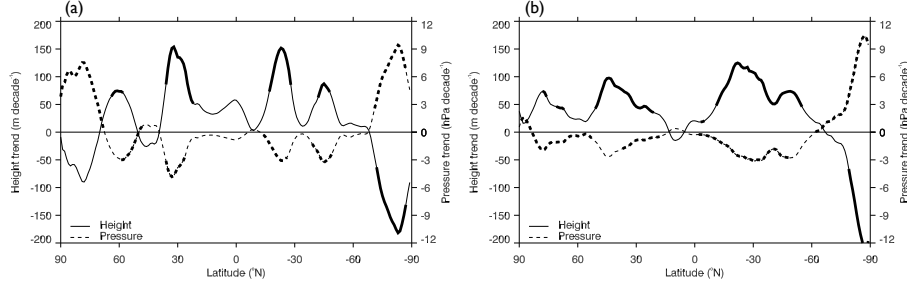
Figure 2: Seasonal-mean zonal-mean blended tropopause height and pressure trends ( \text{m decade}^{-1} and \text{hPa decade}^{-1} ) from ERA-Interim (1989-2007). (a) December to February mean. (b) June to August mean. Bold lines indicate where trends are significant at or above the 5% level.
