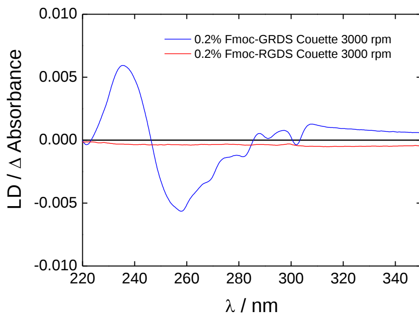
Fig. 4. LD spectra of Fmoc-GRDS and Fmoc-RGDS peptides in water at 0.2 wt% in a 0.5 mm path length Couette alignment cell.
