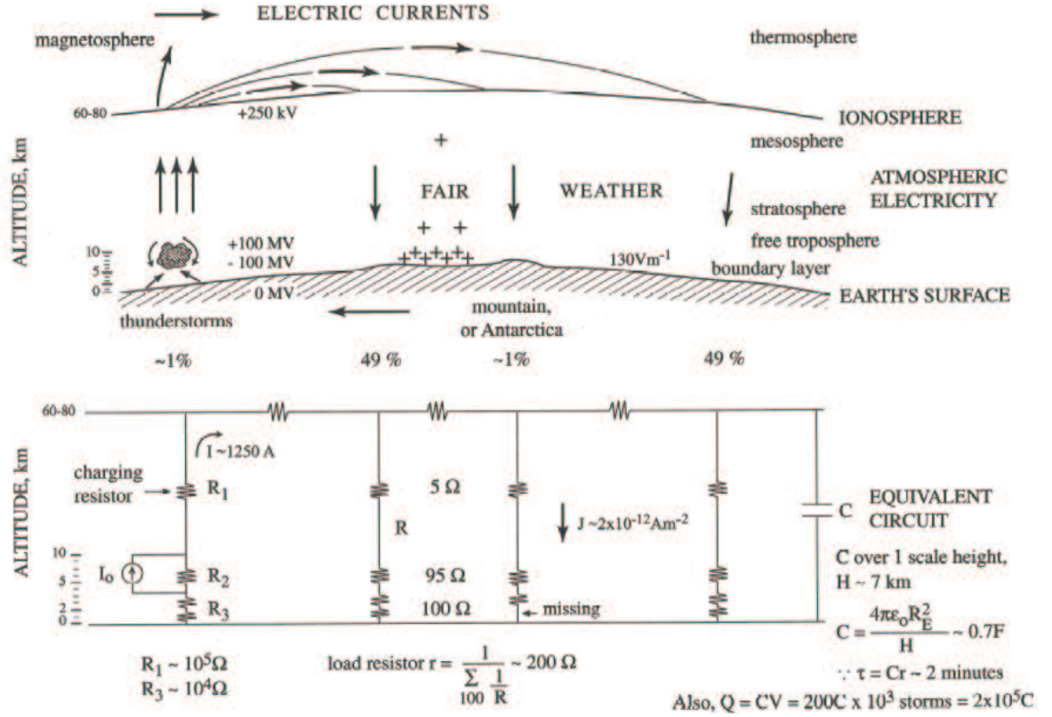
Fig. 3. Taken from Rycroft et al. (2000), the upper panel illustrates a part of the global atmospheric electric circuit. On the left is shown a representative thunderstorm, one of the \sim thousand which are active at all times and which occur over only a small part of the Earth's surface. Huge potential differences are generated inside thunderclouds; acting as giant batteries, they drive an upward (Wilson) current to the ionosphere at an altitude of \sim 80 km. The ionosphere is essentially an equipotential surface at \sim + 250 kV with respect to the Earth's surface, but small currents reach up into the magnetosphere. In fair weather regions remote from thunderstorms, over most of the Earth's surface, downward currents \sim 2 pA/m 2 flow vertically (radially) to the ground. Much more positive charge resides near the Earth's surface than in the stratosphere or mesosphere, as indicated by the density of the + symbols. The lower panel outlines a simple electrical engineering representation of the circuit. Over mountainous regions, the atmospheric columnar resistance is much less than it is elsewhere. Values for the RC (or Cr) time constant are shown at the lower right.
