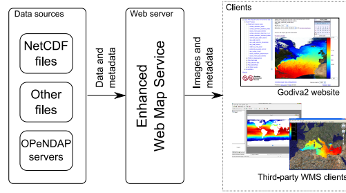
Figure 1. Architecture of the Godiva2 client-server system. Data are read from files on the server or via the OPeNDAP internet protocol. Data are converted to imagery using an enhanced Web Map Service (WMS) and displayed on the Godiva2 website ( http://www.reading.ac.uk/godiva2 ) or any WMS-compatible client.
