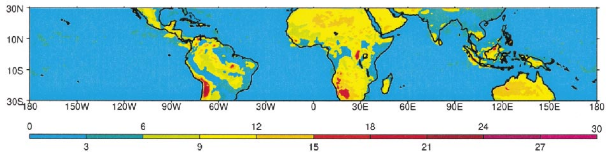
FIG. 8. Diurnal amplitude for the four seasons: DJF, MAM, JJA, and SON.
