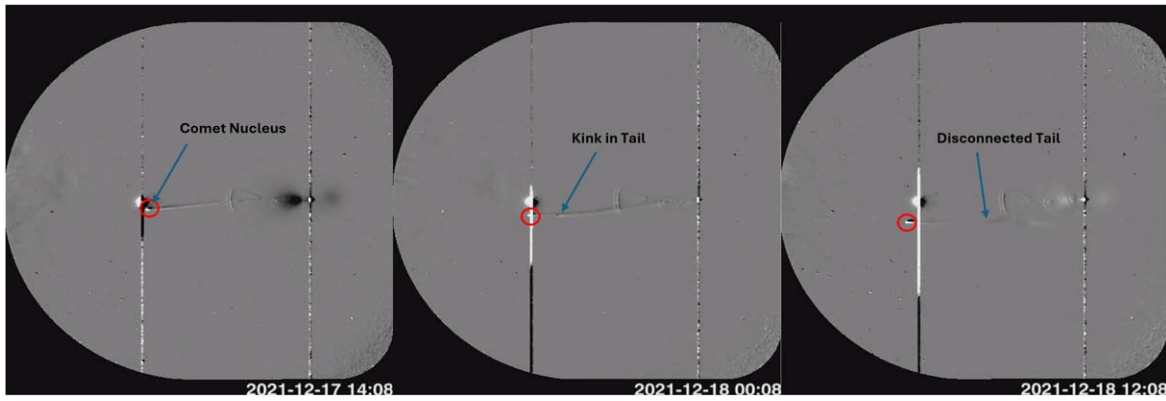
Figure 3. An example of a “disconnection event” that was used in this study. This is a series of three images from the STEREO HI-2 camera. The comet nucleus is circled in red for each image, and the kink and disconnected tail that represent the disconnection event are also labeled. In the left image, you can see the tail of the comet intact. The middle image shows the comet in the process of a tail disconnection, with a clear kink formed in the tail. The final image shows the end of the tail no longer attached to the main tail.
