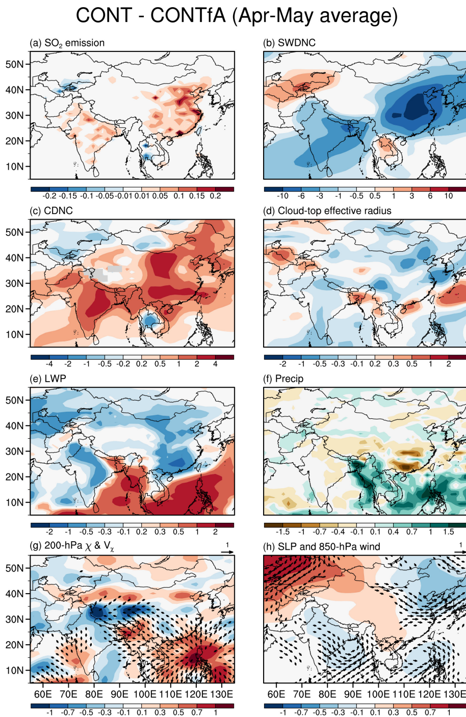
Figure 7. April–May average differences in (a) SO 2 emissions (Tgyr -1 ), (b) clear-sky downward shortwave radiation (SWDNC) (W m -2 ), (c) cloud droplet number concentration (10 10 m -2 ), (d) cloud-top effective radius (μm), (e) liquid water path (LWP; g m -2 ), (f) precipitation (mm d -1 ), (g) 200 hPa divergence (10 6 s -1 , shading) and divergent wind (m s -1 ), and (h) sea-level pressure (hPa) and 850 hPa winds (m s -1 ) between CONT and CONTfA.
