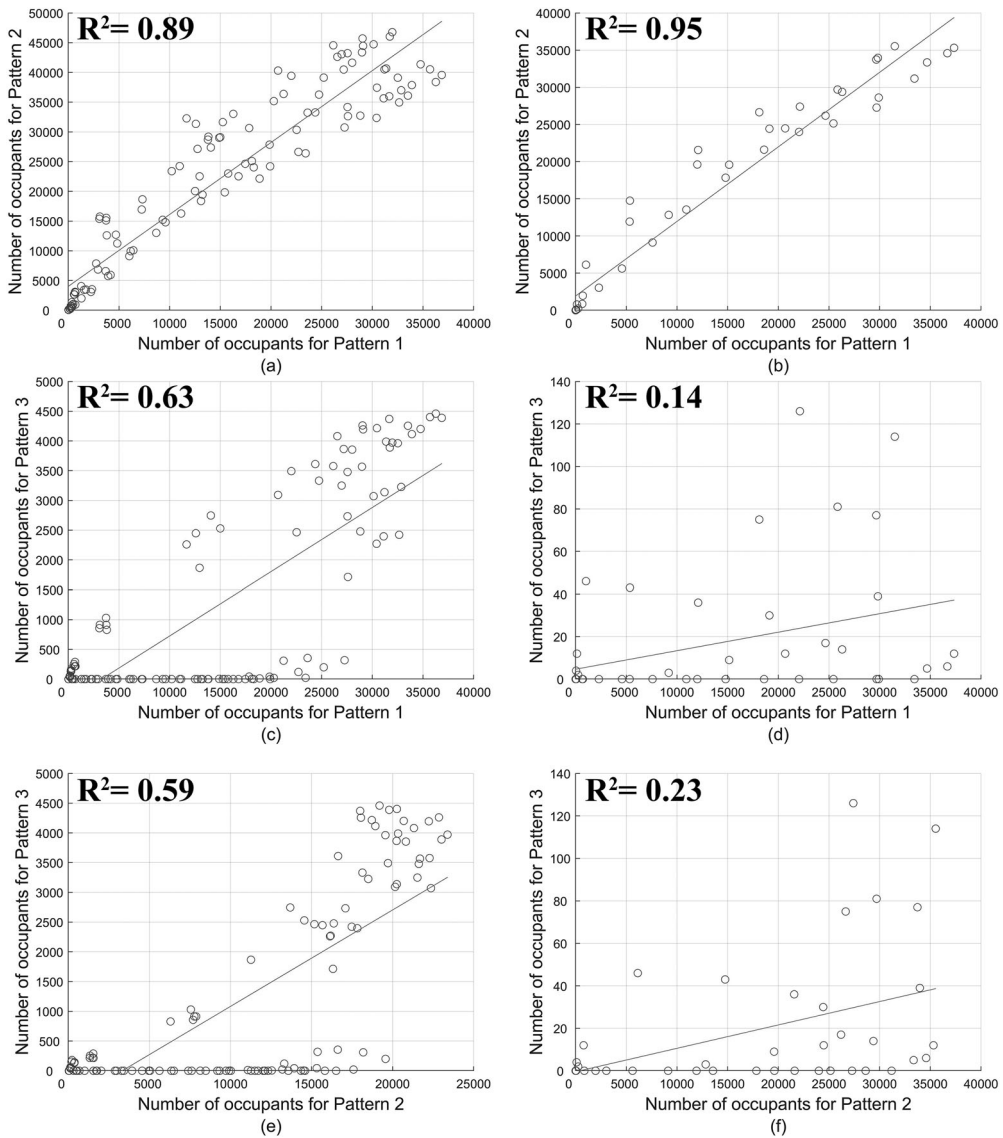
Figure 15. The result of performing the analysis of PCC between Pattern 1 and Pattern 2 during (a) workdays and (b) weekends, Pattern 1 and Pattern 3 during (c) workdays and (d) weekends, and Pattern 2 and Pattern 3 during (e) workdays and (f) weekends.
