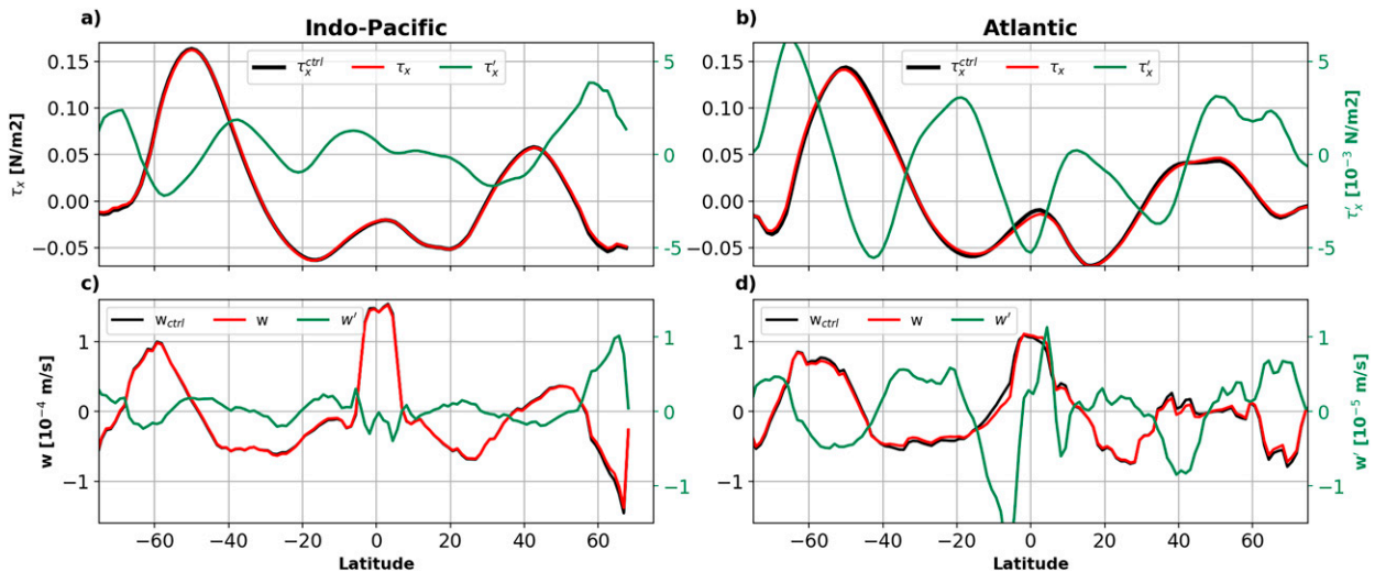
FIG. 8. Zonally averaged zonal wind stress \tau_x for the perturbed (red) and control (black) experiments (left y axis) and their difference (green, right y axis) for the (a) Indo-Pacific and (b) Atlantic Oceans. (c),(d) As in (a) and (b), but for the vertical velocity depth-averaged from the surface to 500 m.
